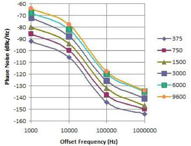
AWG7122C Interleave Phase Noise (typical).
